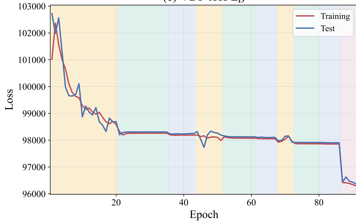
(c) VDF loss L_D
